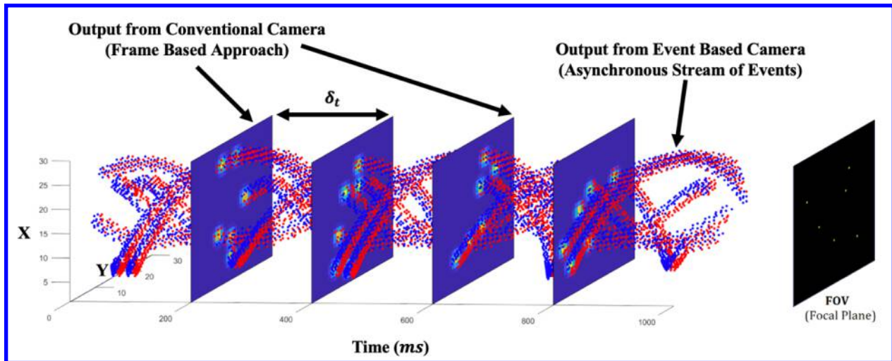
Figure 1 Illustration of the output differences between a conventional camera (frame-based approach) and an event-based camera (asynchronous event stream) for a cluster of particles undergoing circular motion.
