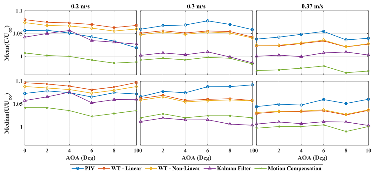
Figure 14 Mean and median U-velocity values for PIV and event-based methods a function of angle of attack at freestream velocities of 0.2 m/s, 0.3 m/s, and 0.37 m/s. Event-based methods replicate global trends observed in PIV, with weighted tracking methods showing the closest agreement.
