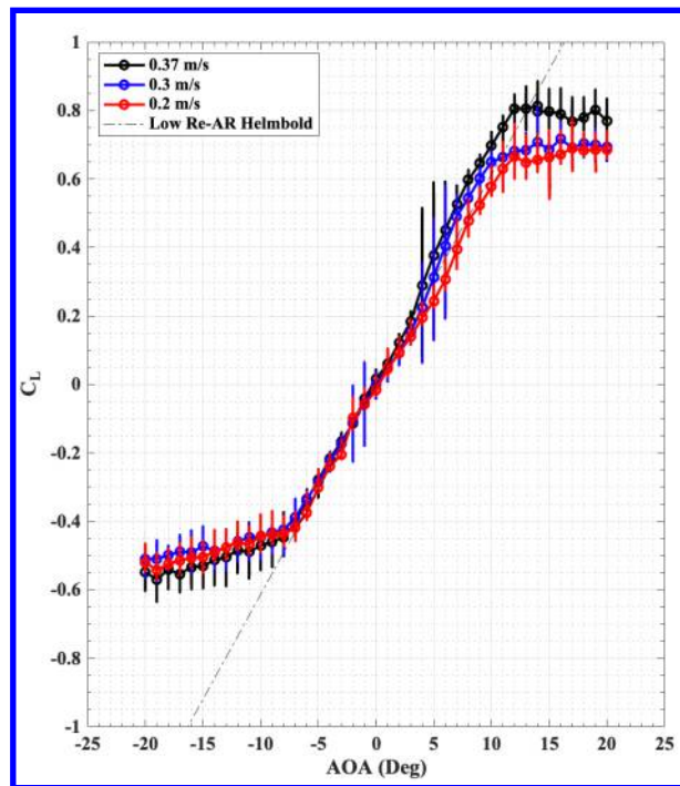
Figure 6 Lift curves for the wing at three velocities corresponding to Reynolds numbers of 17,745 (0.2 m/s), 26,617 (0.3 m/s), and 32,827 (0.37 m/s). The dashed line represents the low Reynolds number corrected lift curve slope.
