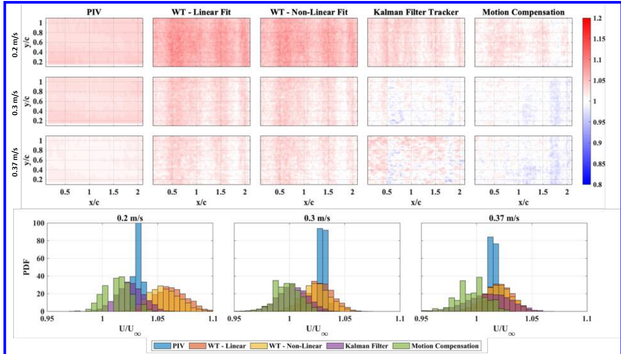
Figure 7 (Top) U-velocity contours at 0.2, 0.3, and 0.37 m/s from PIV and event-based methods. PIV shows smooth gradients, while event-based methods exhibit speckling due to particle-level resolution. (Bottom) Velocity histograms highlight broader distributions for event-based methods and a decreasing bias in mean velocity at higher speeds.
