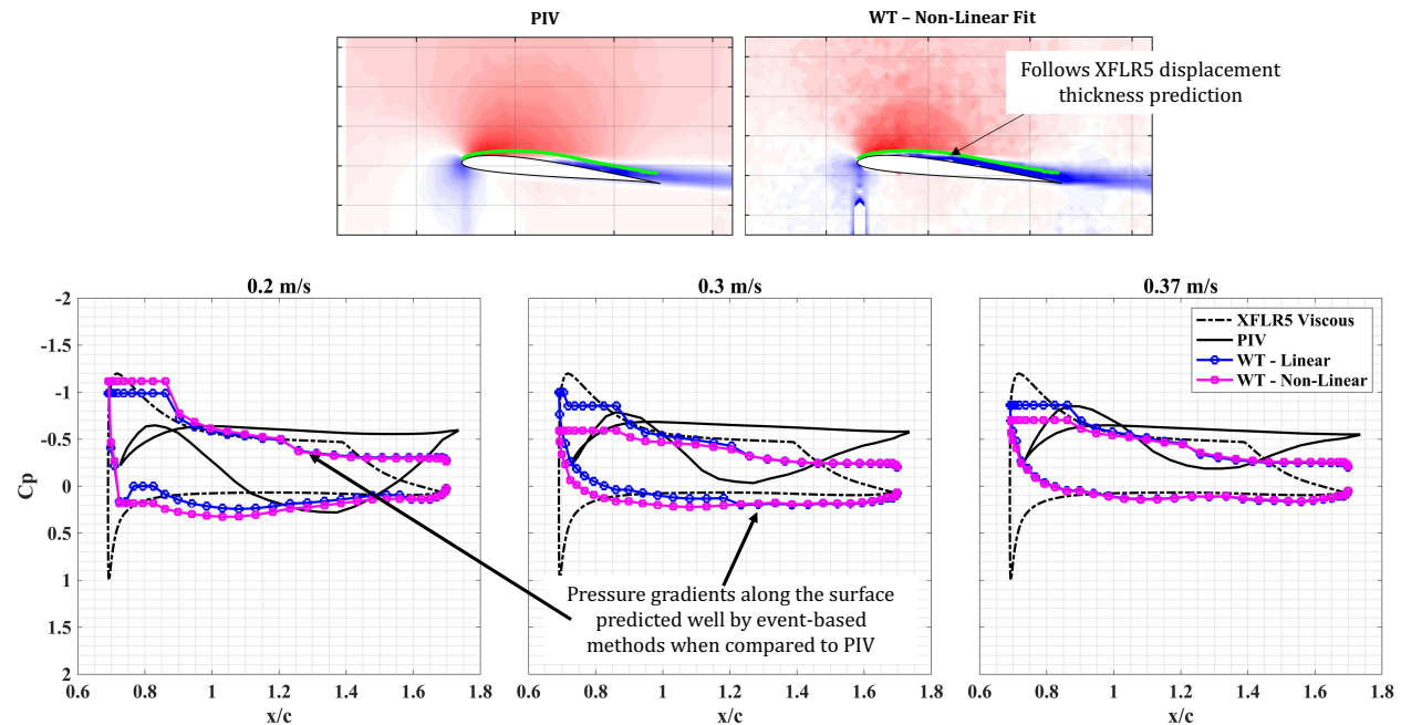
Figure 12 (Top) Normalized U-velocity contours comparing traditional PIV and WT-Non-Linear at \alpha = 4^\circ with XFLR5-predicted displacement thickness (green line). (Bottom) C_p profiles at freestream velocities of 0.2, 0.3, and 0.37 m/s. Event-based methods align more closely with XFLR5 predictions, capturing surface pressure gradients more accurately than PIV.
