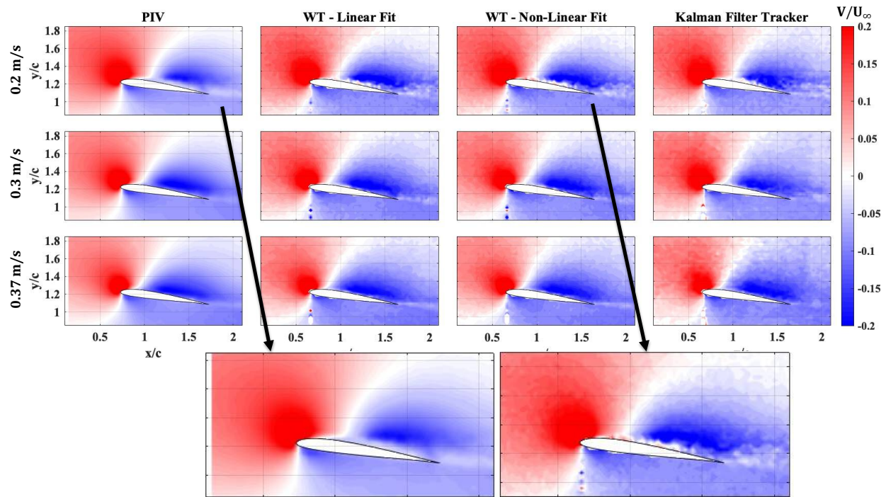
Figure 15 Comparison of normalized V-velocity contours from PIV and event-based methods at \alpha = 8^\circ and freestream velocities of 0.2 m/s, 0.3 m/s, and 0.37 m/s. Event-based methods resolve flow features on the upper surface and in the wake with greater detail than traditional PIV, which smooths gradients due to its window-based approach
