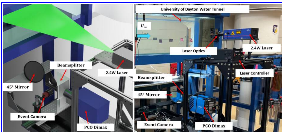
Figure 4 A schematic (left) and actual setup (right) of the event-based and traditional velocimetry system in the University of Dayton Water Tunnel. The setup includes a 2.4W laser, laser optics, a 45° mirror, a 50-50 beam splitter, and two cameras: the Prophesee EVK2 event camera and the PCO DiMax high-speed camera.
