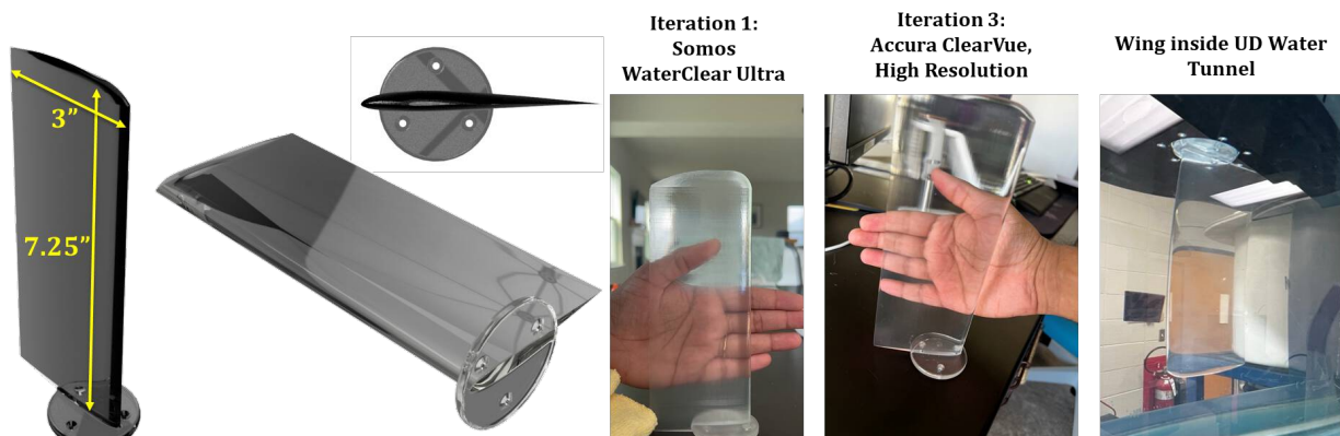
Figure 3 Images showing the design, fabrication, and installation of the SD7003 wing model.
