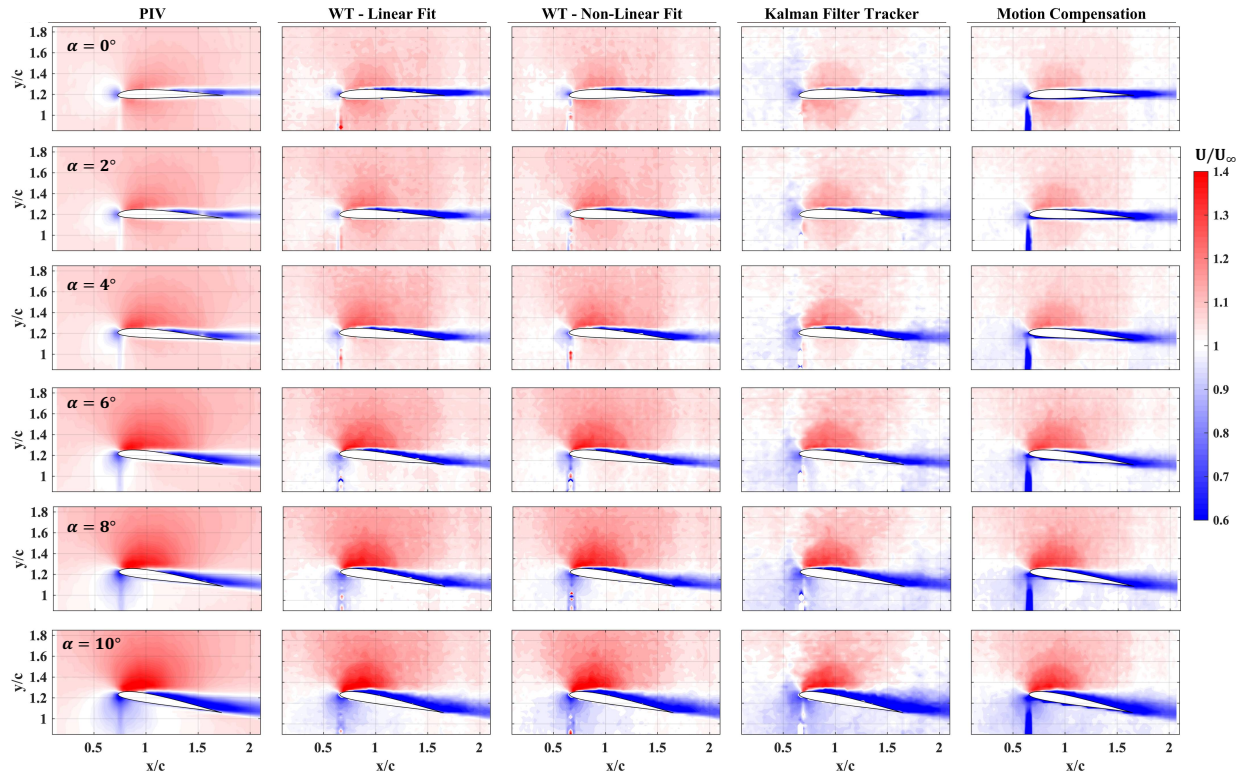
Figure 9 Comparison of normalized U-velocity contours from PIV and four event-based methods (WT-Linear, WT-Non-Linear, Kalman Filter, and Motion Compensation) at angles of attack ranging from \alpha = 0^\circ to \alpha = 10^\circ . PIV shows smooth gradients and clear flow separation, while event-based methods capture similar trends. Weighted tracking methods closely align with PIV results, while Kalman Filter and Motion Compensation exhibit slight biases and shadow artifacts near the leading edge.
