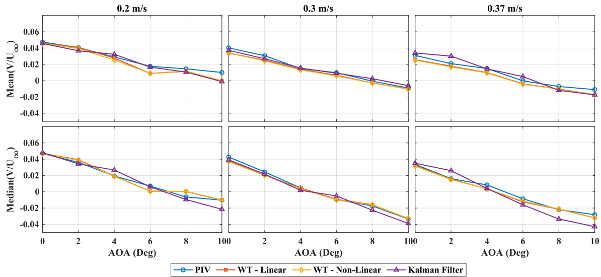
Figure 17 Mean and median V-velocity values for PIV and event-based methods as a function of angle of attack at freestream velocities of 0.2 m/s, 0.3 m/s, and 0.37 m/s. Event-based methods demonstrate trends and magnitudes comparable to PIV, with no observable bias in V-velocity.
