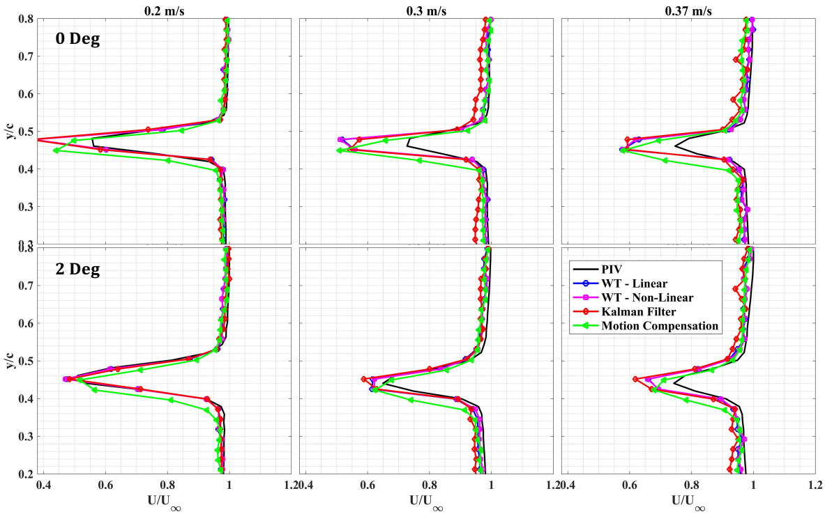
Figure 11 Momentum deficit profiles predicted by PIV and event-based methods (WT-Linear, WT-Non-Linear, Kalman Filter, and Motion Compensation) at freestream velocities of 0.2 m/s, 0.3 m/s, and 0.37 m/s at \alpha = 0^\circ and \alpha = 2^\circ . Event-based methods show consistent performance across the wake and freestream, while PIV results are influenced by frame-rate tuning optimized for the freestream region.
