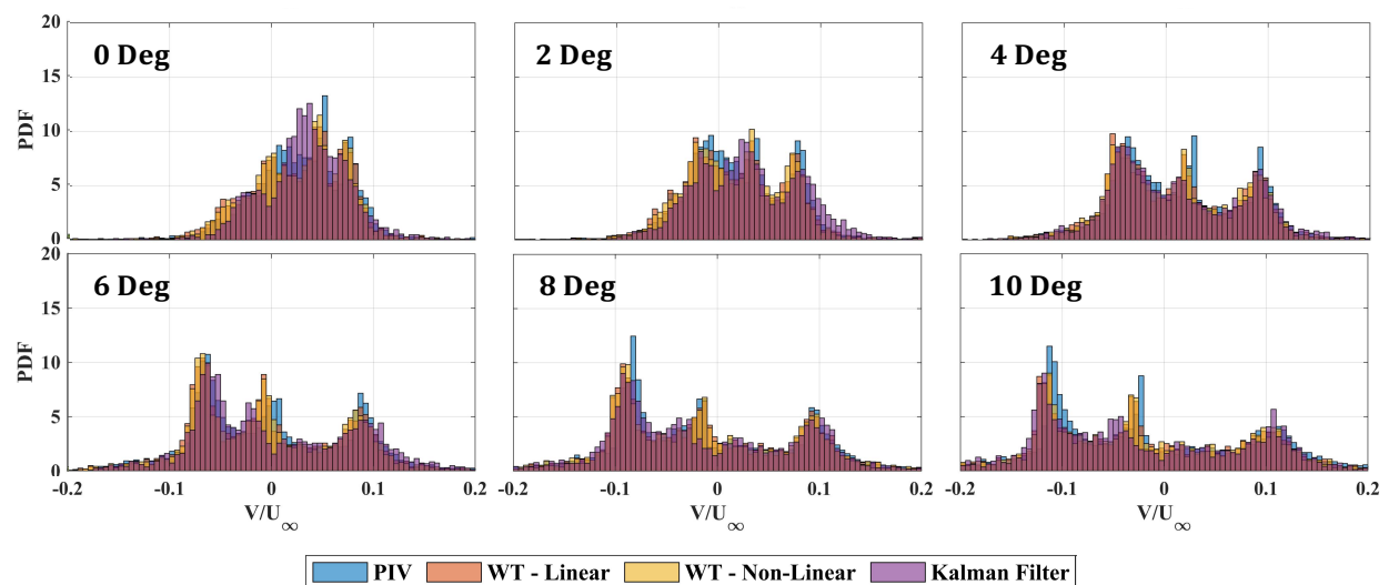
Figure 16 Probability density functions (PDFs) of normalized V-velocity for PIV and event-based methods at angles of attack from \alpha = 0^\circ to \alpha = 10^\circ at 0.37 m/s for U_\infty = 0.37 m/s. Event-based methods show high overlap with PIV distributions, with weighted tracking methods achieving the closest match.
