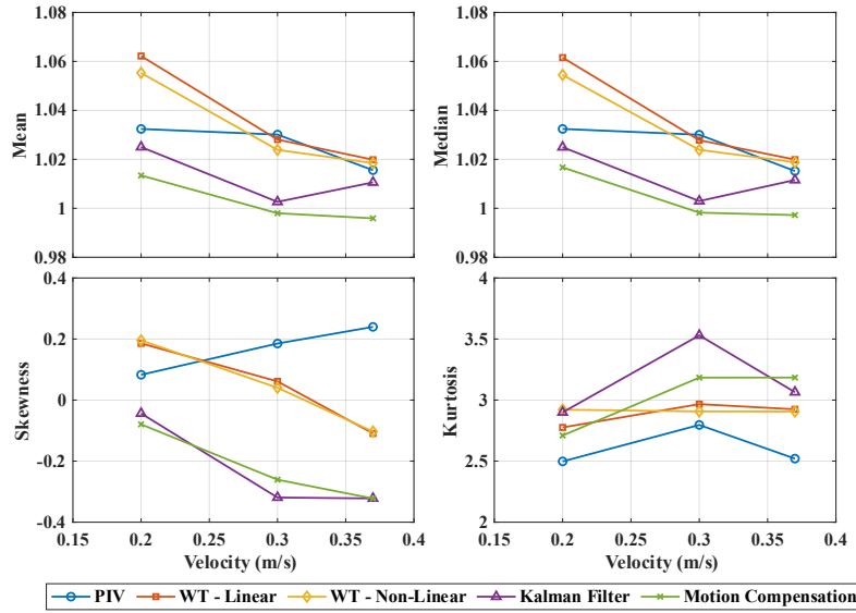
Figure 8 Comparison of mean, median, skewness, and kurtosis for PIV and four event-based algorithms (WT-Linear, WT-Non-Linear, Kalman Filter, and Motion Compensation). WT methods show trends similar to PIV, with stable distributions across velocities. The Kalman Filter demonstrates high sensitivity and variability, while Motion Compensation consistently underestimates and displays skewed distributions.
