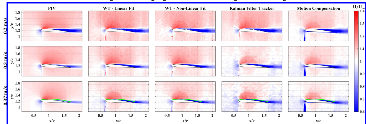
Figure 10 Comparison of normalized U-velocity contours from PIV and event-based methods (WT-Linear, WT-Non-Linear, Kalman Filter, and Motion Compensation) at freestream velocities of 0.2 m/s, 0.3 m/s, and 0.37 m/s, with a fixed angle of attack ( \alpha = 4^\circ )
