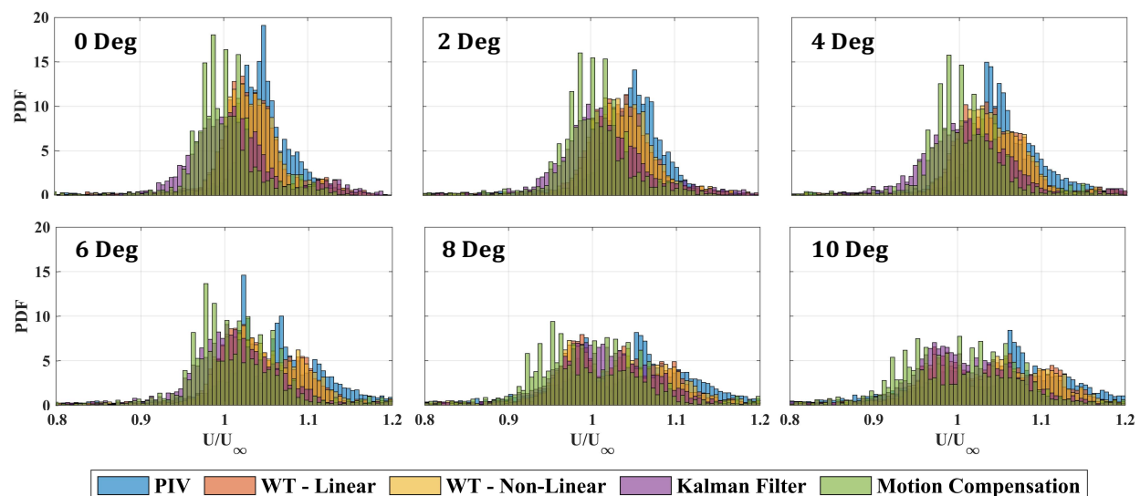
Figure 13 Histograms of normalized U-velocity for PIV and event-based methods at angles of attack from \alpha = 0^\circ to \alpha = 10^\circ at 0.37 m/s. Event-based methods capture global trends with reasonable precision but exhibit slight bias compared to PIV.
